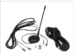
GMAE4248 GPS/Rf integrated antenna with 380-430 MHz frequency range, TETRA and direct mounting.
