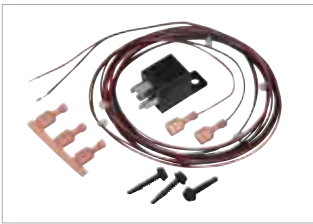
GKN6266 12V power supply cable for GPN6145 and HPN4007.
